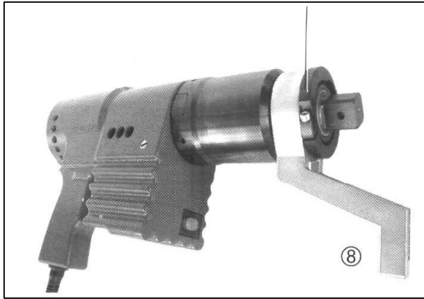
Rubber Safety Ring (DMAR optional)
