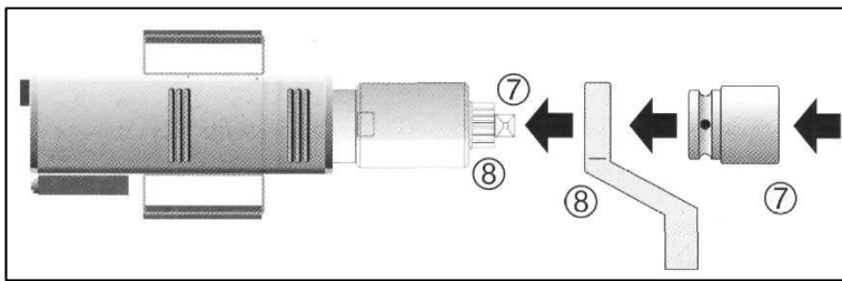
Titan ETite™ ®-DMA Reaction Arm
