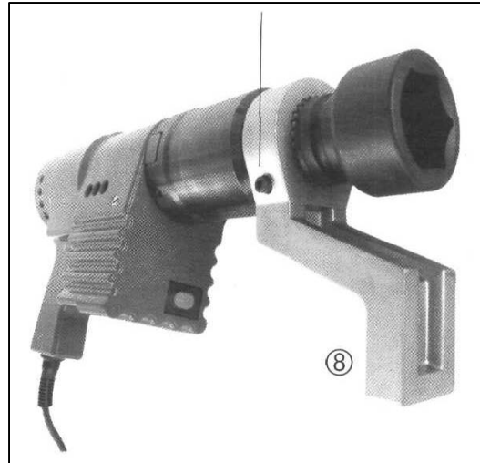
Safety Screw (integrated in the DMA)
